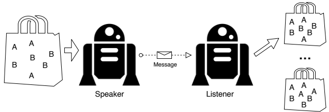
Figure 1: Sketch diagram of the Bag-Select game. The speaker observes a bag of objects of distinct types. The bag can contain a different number of objects of the specific type (here, three As and four Bs). The speaker produces a message, and the listener uses it to select the bag, that the speaker initially observed. The original bag is contained in a set among several other distinct bags, which differ only in the number of As and Bs.
